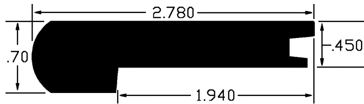
Stair Nosing (H12ZN)
