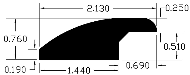
Overlap Reducer (H2ORE)
