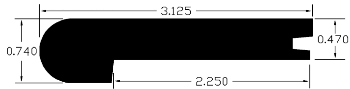
Stair Nosing (H12SN)
