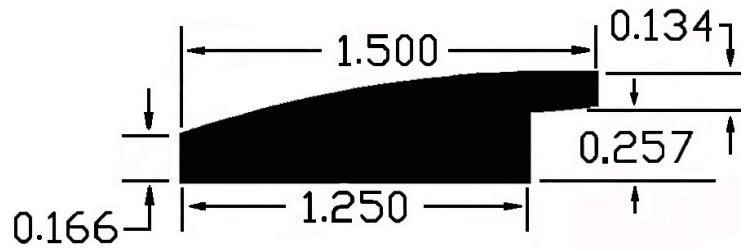
Reducer (H38WR)
