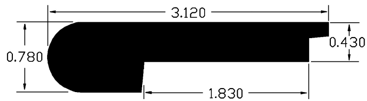
Stair Nosing (H38SN)
