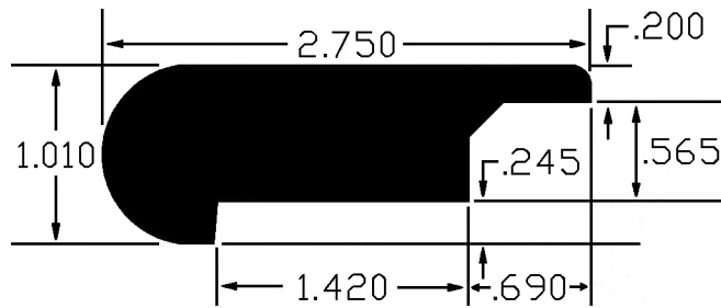
Overlap Stair Nosing (H9UON)
