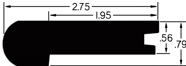
Stair Nosing (H96BN)
