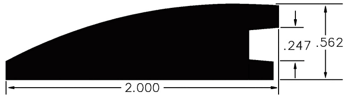
Reducer (H96AR)
