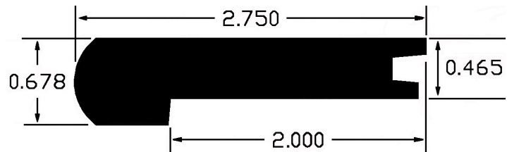
Stair Nosing (H12BN)
