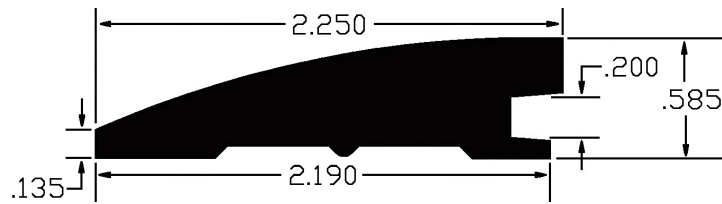
Reducer (H58AR)
