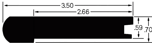
Stair Nosing (H58EN)
