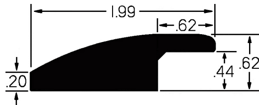
Overlap Reducer (H10RE)
