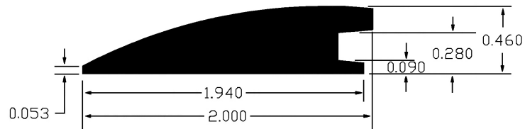
Reducer (H12ZR)
