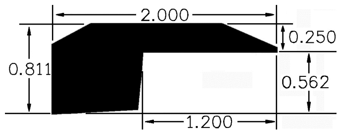
Threshold (H9BAT)
