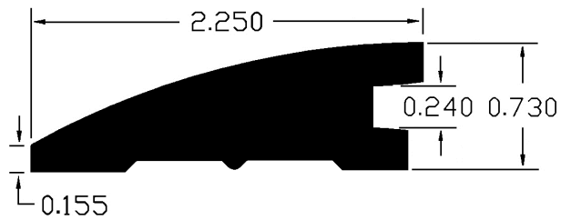
Reducer (H34RE)
