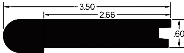
Stair Nosing (H58DN)
