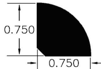
Quarter Round (HQRTR)
