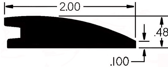
Reducer (H12BR)
